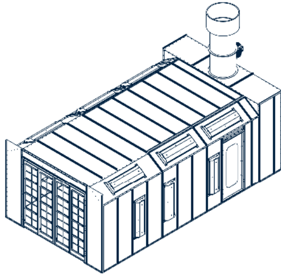
Drawing Accudraft PRO crossflow paint booth. Ductwork and duct cap optional
