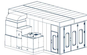
Pitless Downdraft w/Drive Up Ramp
